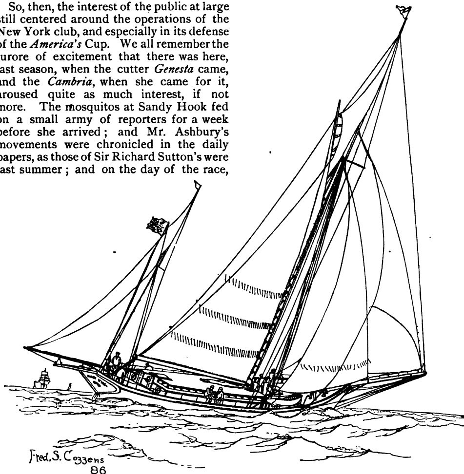
YAWL "WHITE WING." 1
